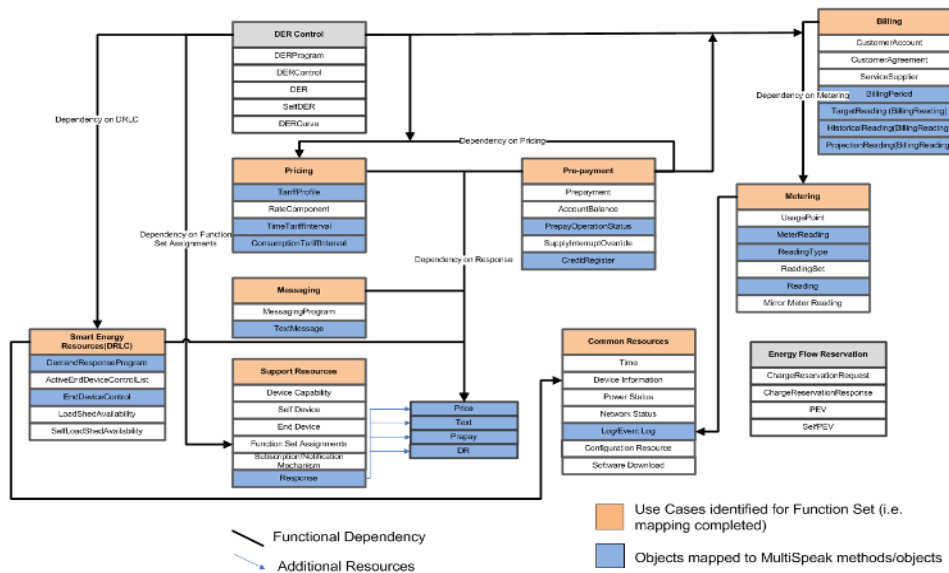
Figure 1 IEEE 2030.5 Function Sets and objects
