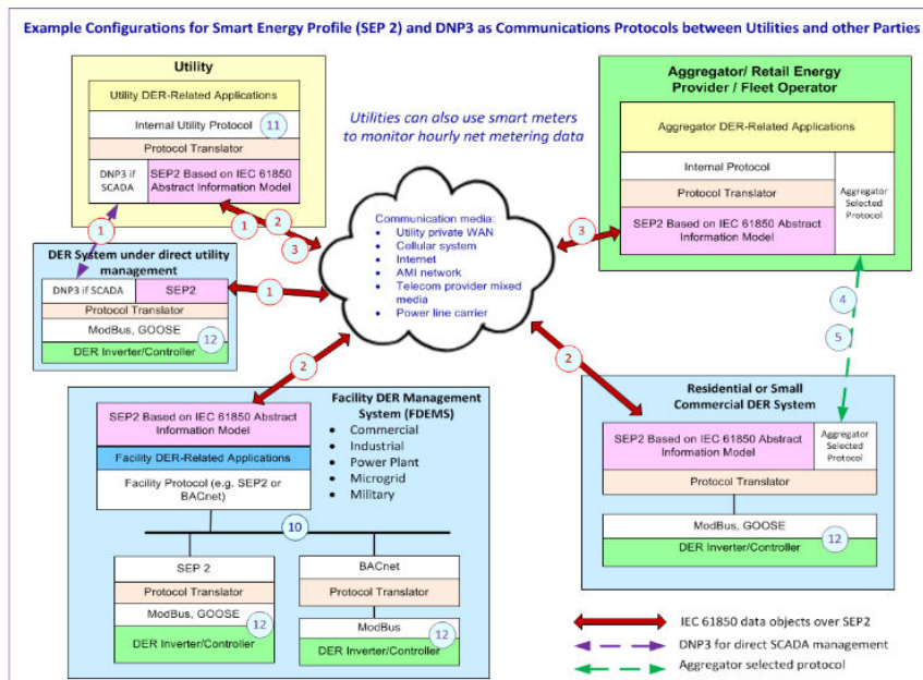
Figure 3: Conceptual Implementation of IEEE 2030.5 (SEP2) Communications with DER 12
