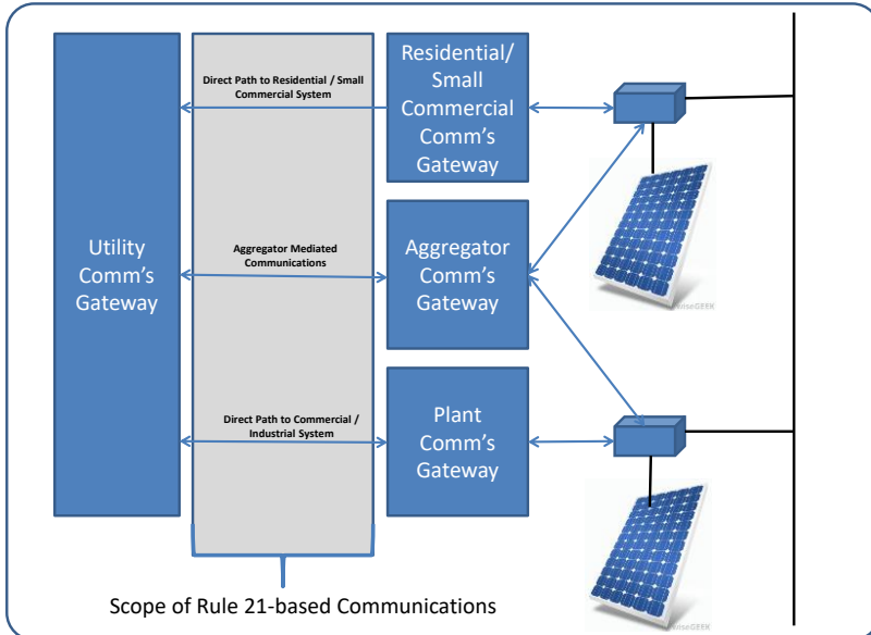
Figure 2: Scope of CA Rule 21 DER Communications
